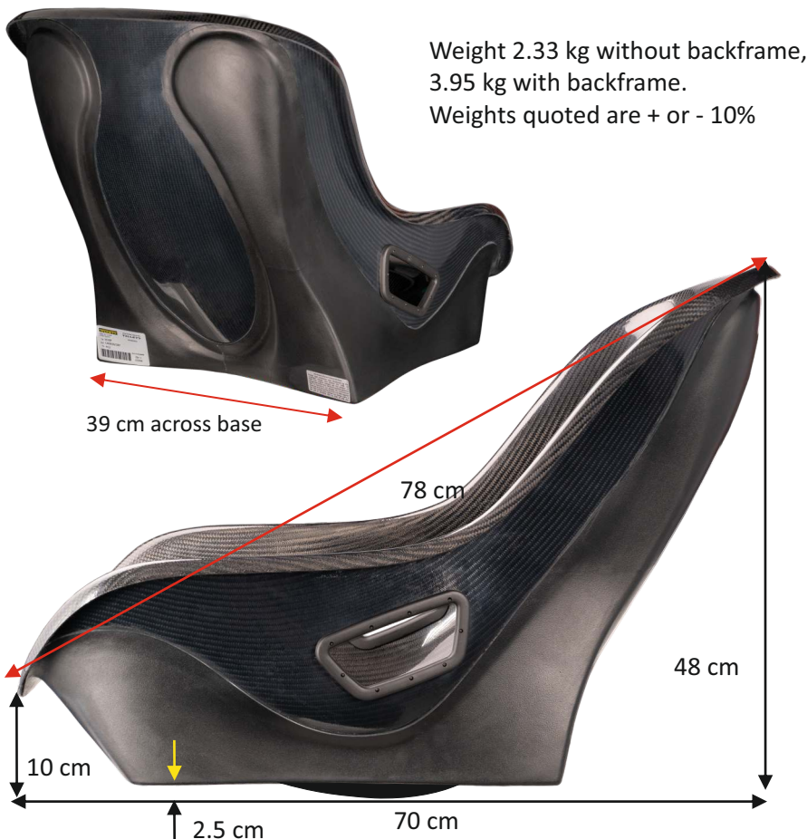
W2i carbon GRP with back frame.
